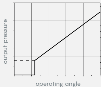
STRAIGHT TYPE CURVE (example)
