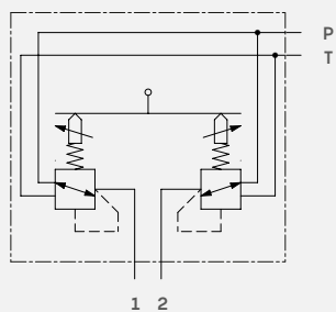
HYDRAULIC CIRCUIT
